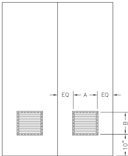
ELEVATION-B LOUVER TYPE X ONLY BOTH DOORS IDENTICAL
