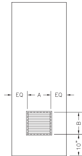
ELEVATION-C LOUVER TYPE I THRU VII
